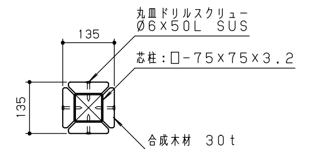
柱断面图 S = 1 / 10
